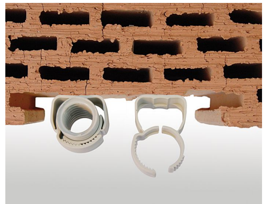
An innovative product for sub-plaster mounting - the Buried Clamp Automatic USA. A quick push is enough to affix the clamp to the pipe.
